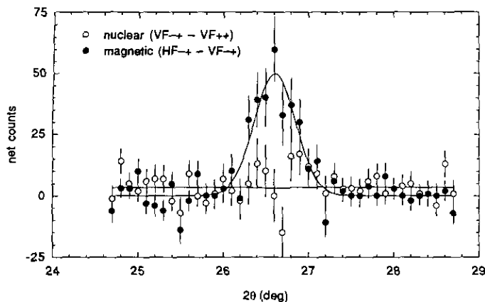
FIG. 1. Compilation of polarized beam diffraction pattern around the 011 reflection of \text{YBaCuCoO}_5 . The closed symbols ( \bullet ) are the difference between the horizontal and vertical field spin flip cross sections, which gives the magnetic component of the reflection. The open symbols ( \circ ) are the difference between the vertical field spin flip and nonspin flip cross sections, which is the coherent nuclear Bragg component of the reflection. The 011 reflection is purely magnetic, with no nuclear structure contribution.
