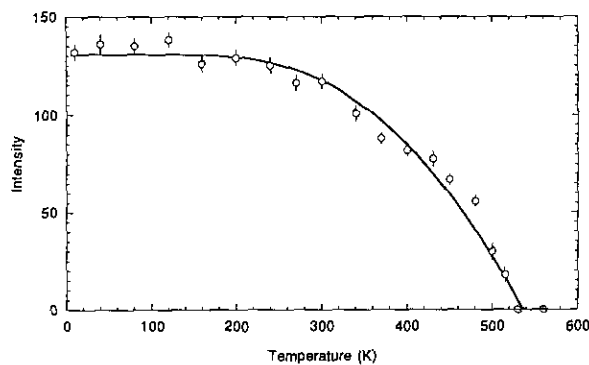
FIG. 2. Intensity of the 011 reflection of \text{YBaCuCoO}_5 as a function of temperature. The solid line is a fit to a simple mean-field model. The value of T_N obtained from the fit is T_N = 536(3) \text{ K} .
